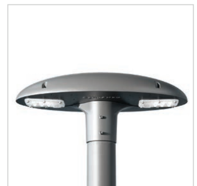
The luminaire is mounted on a Ø48-60mm spigot by tightening two M8 screws.
